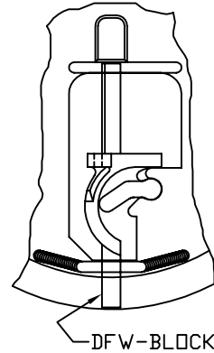
PLAIN KEY LOCK OPTION PART #: DFW18AMRX-1BA-LID
