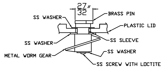
DFW-SCREWWORM ASSEMBLY
